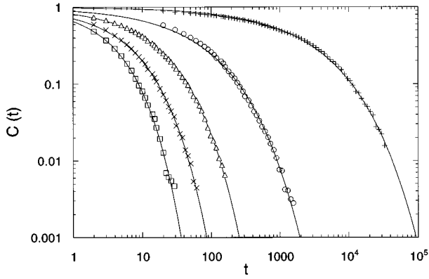
FIG. 3. The correlation function for various temperatures: T=2.8 ( \square ), and T=2.4 ( \times ), T=2.0 ( \triangle ), T=1.6 ( \circ ), and T=1.2 ( + ). The lines are stretched exponential fits.
