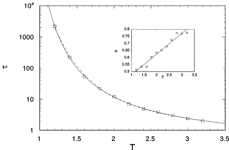
FIG. 4. The relaxation time as a function of the temperature together with the Vogel-Fulcher fit (solid line) and the \exp(B/T^2) fit (dashed line). The inset shows the temperature dependence of the exponent b .
