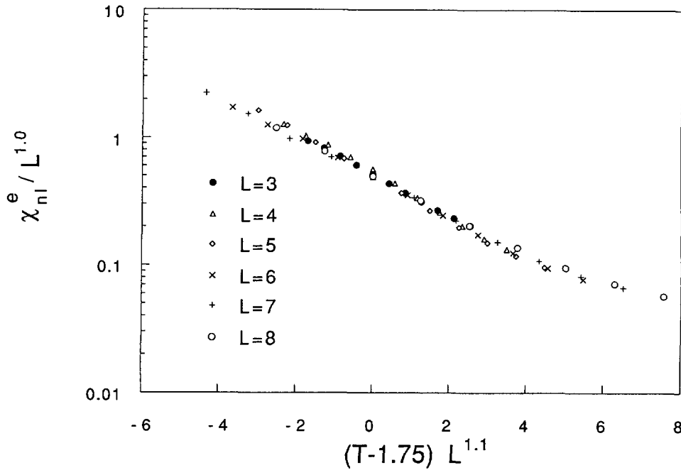
Fig. 8. — Finite-size scaling for \chi_n^e at h = 0.3 .
