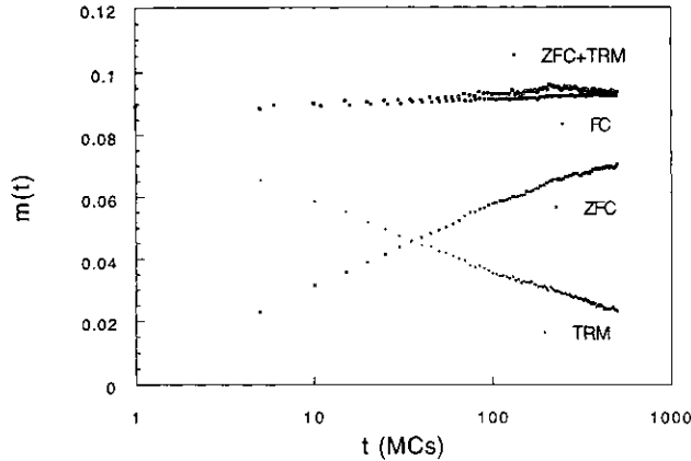
FIG. 1. Zero-field-cooled magnetization and thermoremanent magnetization and their sum for waiting time t_w = 100 , and the magnetization corresponding to a constant field. For all the curves D = 17 , T = 0.2 , and h = 0.1 .
