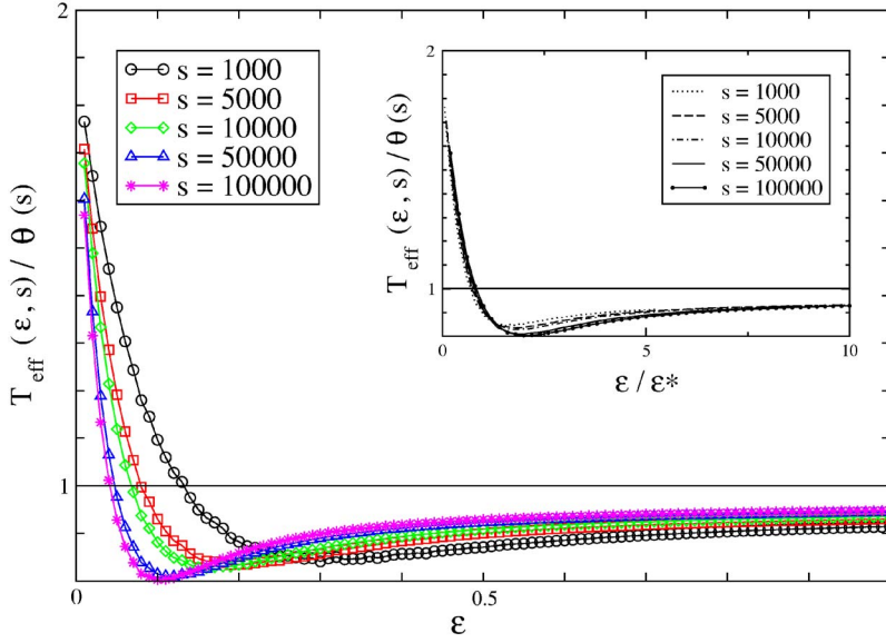
FIG. 7. (Color online) The dependence of the effective temperature (in time domain) as a function of the value of \epsilon for the same system as in Fig. 3 with 100 types of oscillators with \epsilon values equally spaced and uniformly distributed between 0.01 and 1.00. Data is shown for different waiting times at zero temperature. In the inset we show the scaling of the effective temperature with the threshold energy \epsilon^* .
