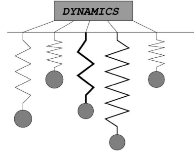
FIG. 1. Schematic picture of a system of independent oscillators with different spring constants. The thickness of the springs represents different values for the spring constants. The motion of the oscillators is not independent due to the coupling induced by the Monte Carlo dynamics (represented by the top rectangular box with the heading “dynamics”).
