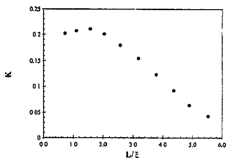
Figure 6. K as a function of L/\xi .
