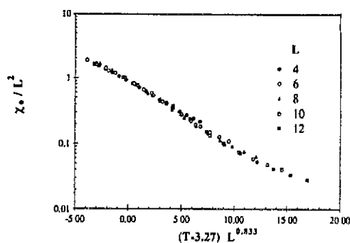
Figure 2. The scaled overlap susceptibility \chi_0/L^2 plotted against the scaled reduced critical temperature (T - T_c) L^{1/\nu} .
