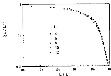
Figure 4. The rescaled \chi_0 as a function of L/\xi . This scaling is compatible with a singularity at T = 0 .
