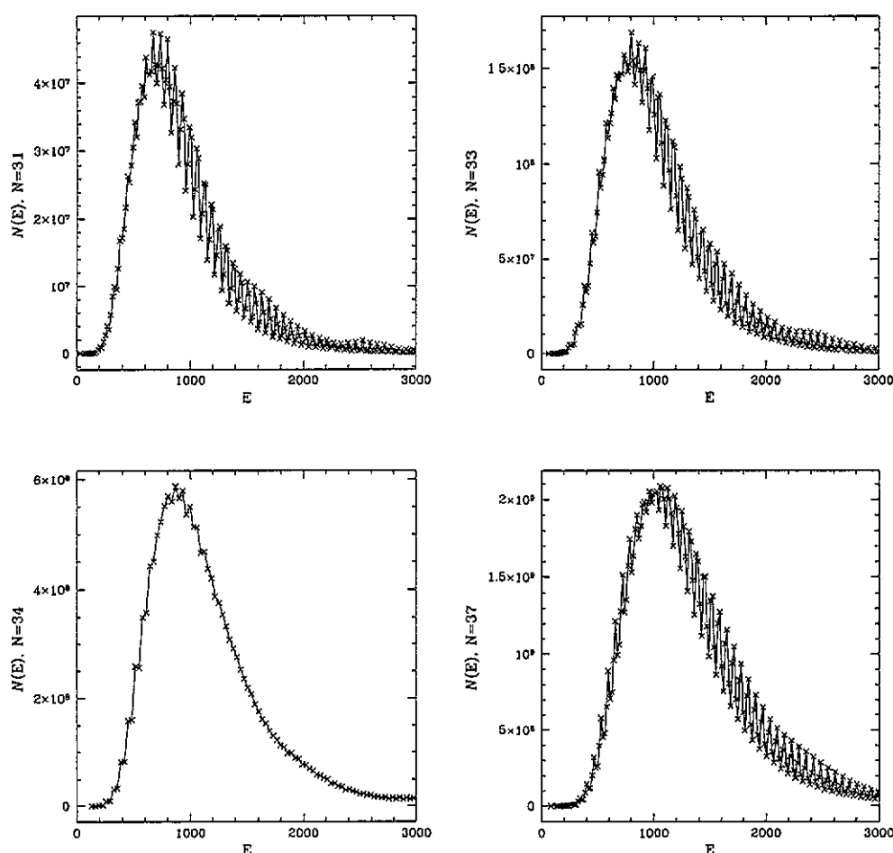
Figure 2. N(E) , the number of configurations of energy E as a function of E . (a) N = 31 (a good prime); (b) N = 33 (of the form 4n + 1 , non-prime); (c) N = 34 (of the form 4n + 2 ); (d) N = 37 (of the form 4n + 1 , prime).
