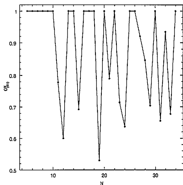
Figure 5. O_{(0,1)}^M as a function of N .
