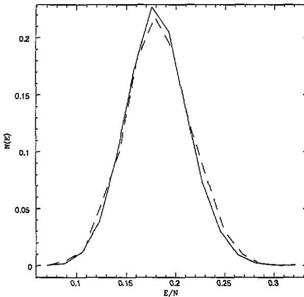
Figure 13. The number of solutions of the T = 0 mean-field equations of a given energy as function of the energy for N = 56 , where (2N + 1) is prime (broken curve) and for N = 57 , where (2N + 1) is not prime (full curve).
