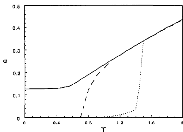
Figure 10. Energy of the cosine model versus T , for prime values of (2N + 1) . The full curve is for decreasing T starting from a random configuration (and is the same for the two lattice sizes), while the broken curve starts from a true ground state for increasing T , N = 44 , and the dotted curve is for increasing T , N = 806 .
