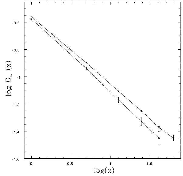
FIG. 1. \log[\tilde{G}_\infty(x)] \log(x) , where \log is the natural logarithm. The upper line is from cooling, the lower one from the normal dynamics (see the text for details).
