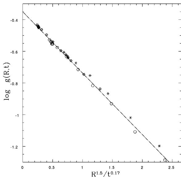
FIG. 2. The logarithm of the Binder cumulant for the box overlap versus rescaled ratio of time and distance. Stars are for R = 2 , hexagons are for R = 3 , and asterisks for R = 4 . The straight line is only to guide the eye.
