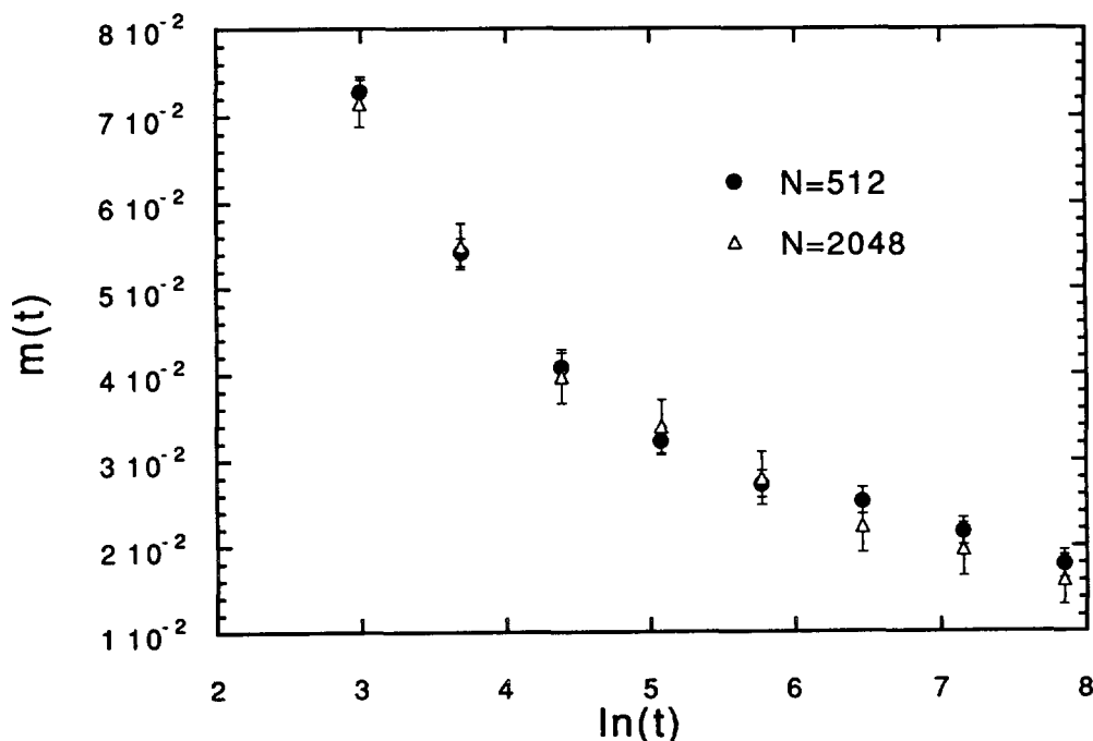
Fig. 5. — Remanent magnetization in the SK model with discrete \pm 1 couplings at T = 0.4 . Data is shown for two sizes N = 512, 2048 and 500 and 40 samples respectively. Remanent magnetization is measured each 10 Monte Carlo steps in a total run of 2 560 and averaging over 8 exponentially increasing periods of time.
