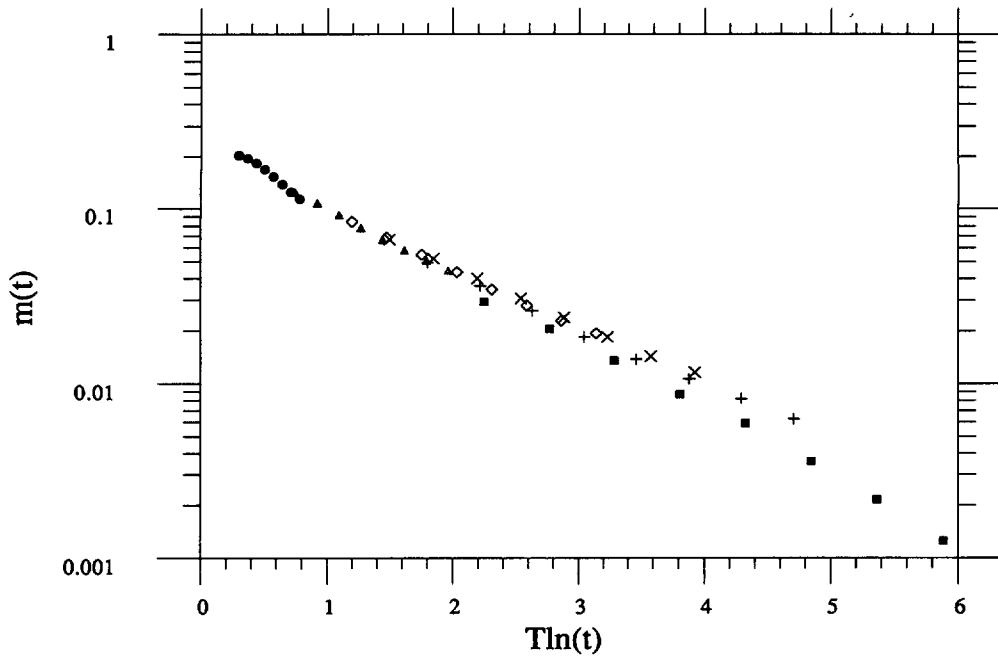
Fig. 4a. — Remanent magnetization in the hypercube model with discrete \pm 1 couplings ( D = 15 ). Data are averaged over 10 samples. The symbols are : ( \bullet ) T = 0.1 , ( \Delta ) T = 0.25 , ( \diamond ) T = 0.4 , ( \times ) T = 0.5 , (+) T = 0.6 , ( \square ) T = 0.75 .
