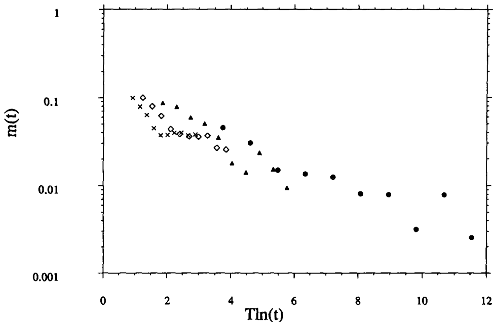
Fig. 3a. — Remanent magnetization in the random lattice model with discrete \pm 1 couplings and coordination number z = 4 . Data are shown for N = 100\,000 and 1 sample. The symbols are : (●) T = 1.25 , (Δ) T = 0.625 , (◇) T = 0.42 , (×) T = 0.3 .
