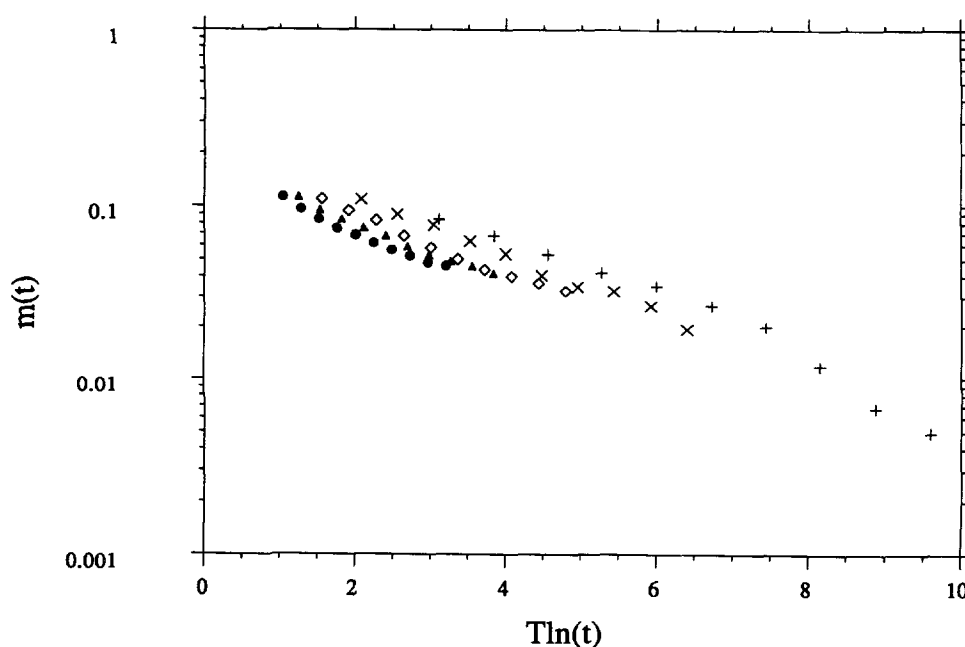
Fig. 3c. — Remanent magnetization in the random lattice model with discrete \pm 1 couplings and coordination number z = 6 . Data are shown for N = 50\,000 and 1 sample. The symbols are : (●) T = 0.35 , ( \Delta ) T = 0.41 , ( \diamond ) T = 0.52 , ( \times ) T = 0.69 , (+) T = 1.04 .
