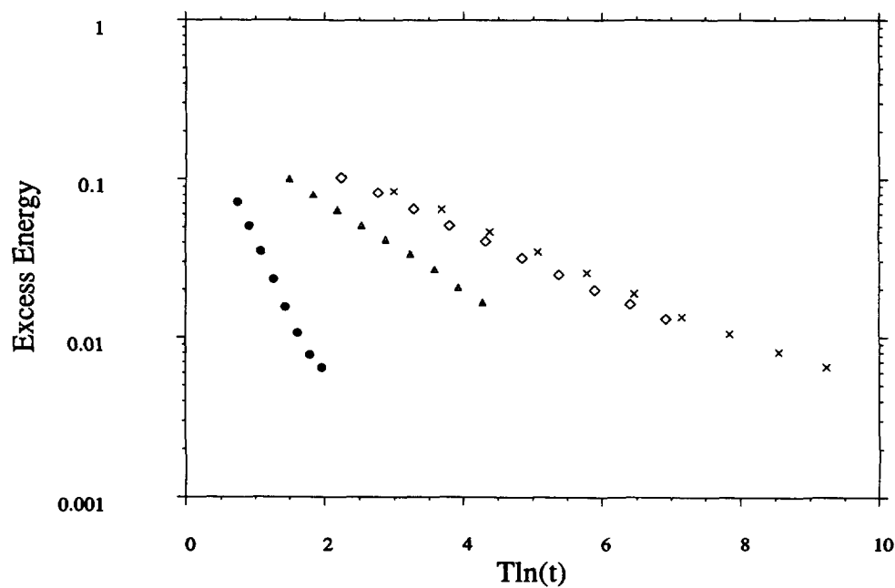
Fig. 1b. — Decay of the excess energy in the binary 3-d Ising spin glass with L = 39 and 1 sample. The same temperatures and symbols like in figure 1a.
