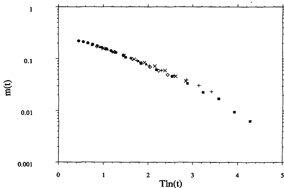
Fig. 3b. — Remanent magnetization in the random lattice model with continuously distributed Gaussian couplings and coordination number z = 4 . Data are shown for N = 100\,000 and 1 sample. The symbols are : (●) T = 0.15 , ( \Delta ) T = 0.25 , ( \diamond ) T = 0.286 , ( \times ) T = 0.33 , (+) T = 0.4 , ( \square ) T = 0.5 .
