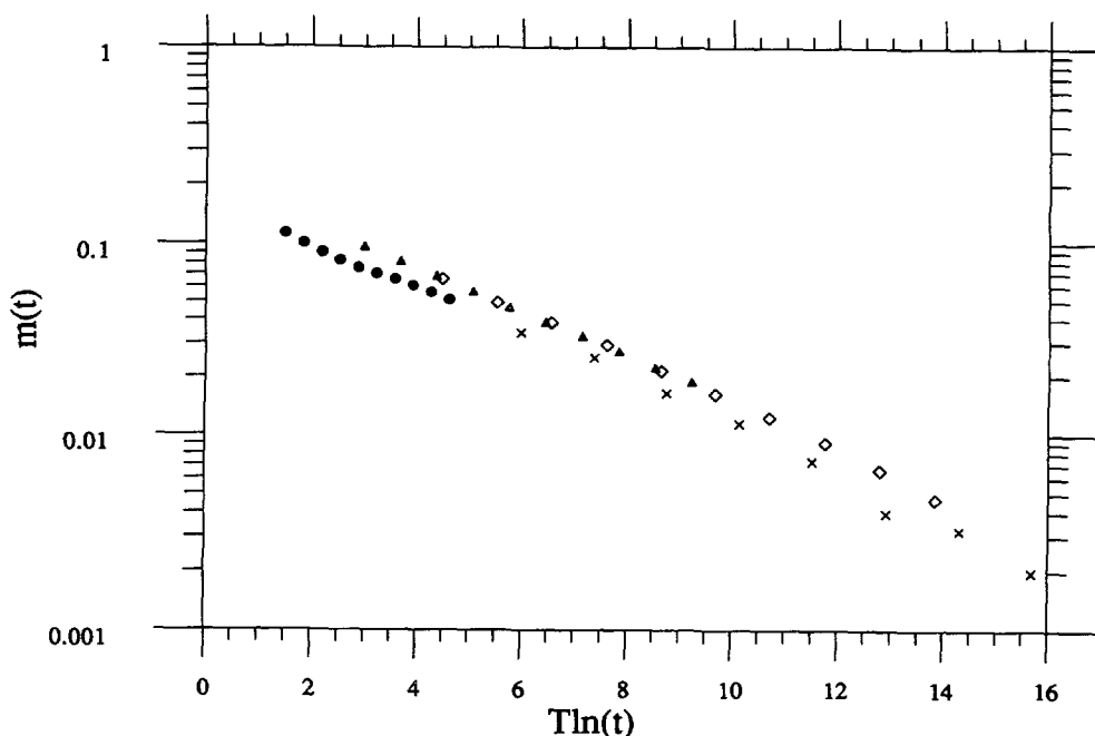
Fig. 2a. — Decay of the remanent magnetization in the binary 4-d Ising spin glass with L = 10 and 8 samples at four different temperatures : ( \bullet ) T = 0.5 , ( \Delta ) T = 1.0 , ( \diamond ) T = 1.5 , ( \times ) T = 2.0 .
