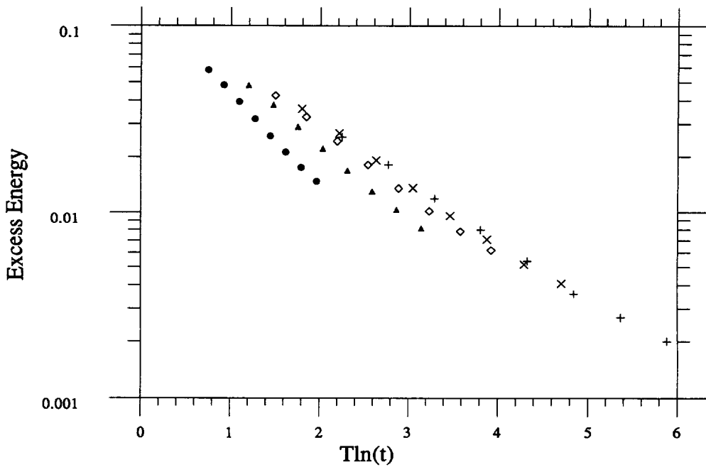
Fig. 4b. — Excess energy in the hypercube model with discrete \pm 1 couplings ( D = 15 ). Data are averaged over 10 samples. The same temperatures and symbols like in figure 4a. However, data is not shown for T = 0.75 because of large error bars when approaching the mean-field critical temperature T_c = 1 .
