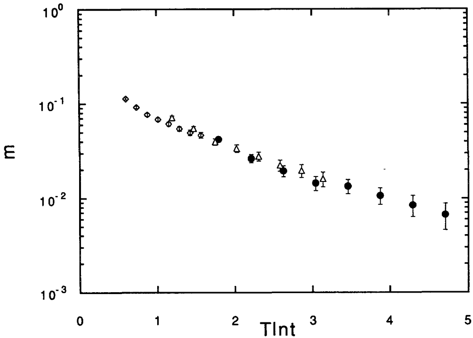
Fig. 6. — Remanent magnetization in the SK model ( N = 2\,048 ) at three different temperatures. Data is averaged over 40 samples. The symbols are : (●) T = 0.6 , ( \Delta ) T = 0.4 , ( \diamond ) T = 0.2 .
