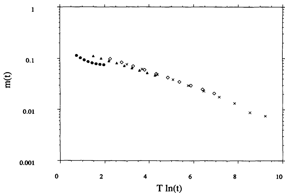
Fig. 1a. — Decay of the remanent magnetization in the binary 3-d Ising spin glass with L = 39 and 1 sample at four different temperatures : (●) T = 0.25 , ( \Delta ) T = 0.5 , ( \diamond ) T = 0.75 , ( \times ) T = 1.0 .
