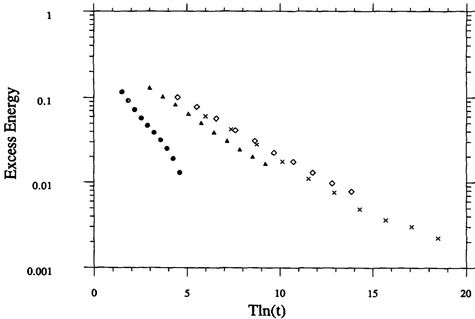
Fig. 2b. — Decay of the excess energy in the binary 4-d Ising spin glass with L = 10 and 8 samples. The same temperatures and symbols like in figure 2a.
