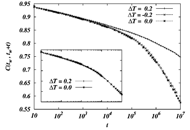
FIG. 2. Correlation relaxation in temperature cycling experiments. In the inset we have used temperatures and time scale ratios similar to the experimental ones (see text for details) and we do not see any difference with respect to the reference curve. In the main part we show the results for a large perturbation both in temperature, \Delta T = \pm 0.2 , and in times, t_{w2} = t_{w1} + t_{w3} = 10^6 . It is clear that for both positive and negative cycles the system is more thermalized with respect to the reference system where t_w = 10^6 .
