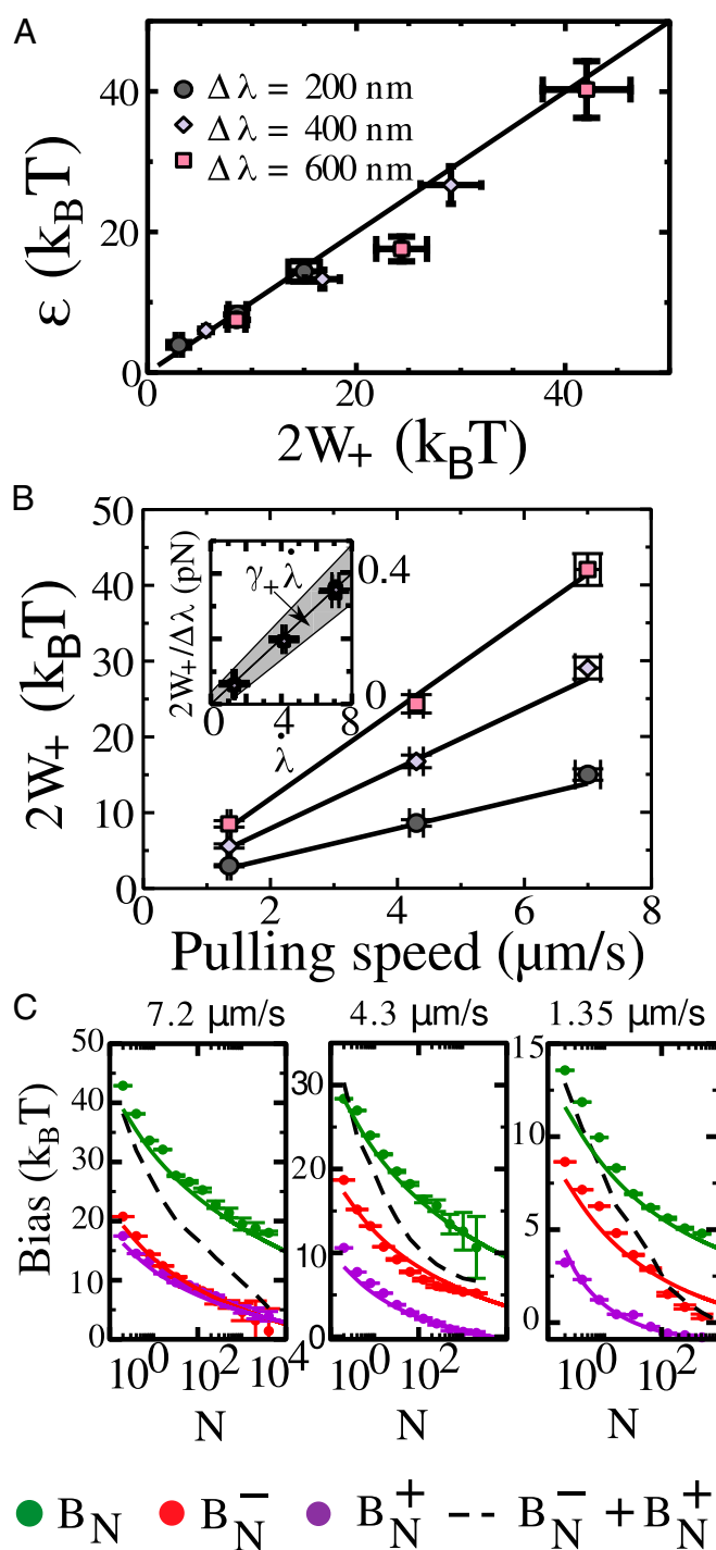
Fig. 3. Bias in unidirectional free-energy estimators. (A) Error ( \epsilon ) on free-energy estimates (Eq. 12) committed by using JE for W' . Circles, diamonds, and squares refer to excursions of 200 nm, 400 nm, and 600 nm. Three different pulling speeds were considered in each case. Note that in this case work is evaluated over closed cycles ( \Delta G = 0 ) and the error is defined as \epsilon = -\beta^{-1} \log(e^{-\beta W'}) . (B) \langle W^+ \rangle displays a bilinear dependence on pulling speed \lambda and (Inset) \Delta\lambda as expected from Eq. 17. Solid lines are linear fits to the experimental results, which contain a single fitting parameter. The shaded area (Inset) corresponds to the region within 1 SD from the expected value of \langle W^+ \rangle based on equilibrium measurements of \gamma_+ (SI Text, sections S4 and S5). (C) Experimental bias measurements from the cycles shown in Fig. 1C. The plots show the bias (Eqs. 22 and 23) as a function of the number of work measurements, N . The three plots correspond to different pulling speeds (7.2 \mu m/s , 4.3 \mu m/s , and 1.35 \mu m/s ). Interestingly B_N^- \ll B_N , which guarantees faster convergence of free-energy estimates. Moreover, B_N is also larger than
