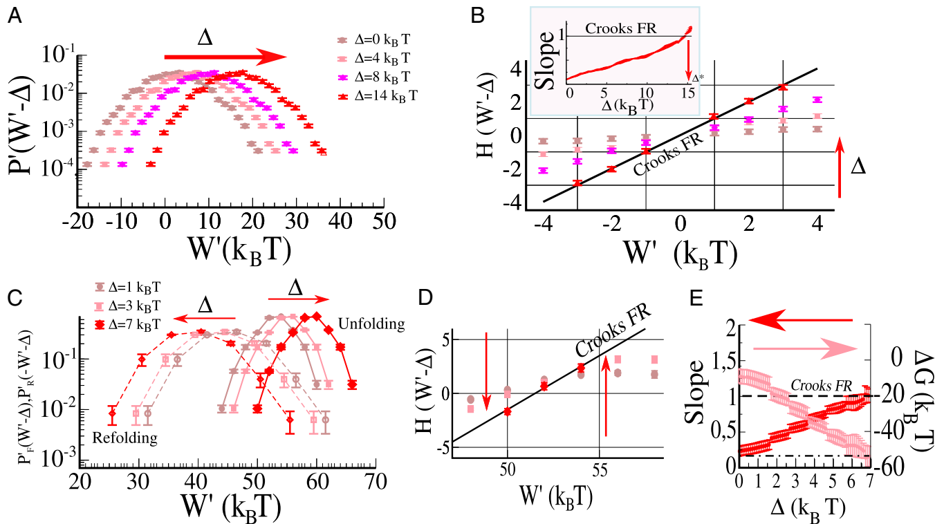
Fig. 5. Inference of P(W) from partial work measurements in the symmetric case. (A) The distribution P(W') in the case of the dsDNA tether, for the work measured in the wrong trap, W' . The distribution does not fulfill the CFR. To recover the correct work distribution P(W) , W' is shifted by a constant amount \Delta . The shifted distribution is tested for the CFR by defining the function H(W') = \log(P(W' - \Delta)/P(-W' - \Delta)) . The prediction by the CFR is H(W') = \beta(W' - \Delta G) . (B) Evolution of H(W') as a function of W' for different values of \Delta . The value \Delta^* for which the slope of H(W') is equal to 1 (work being measured in k_B T units) determines the correct work distribution P(W) ( \Delta \approx 15 , Inset ). (C) In the case of bidirectional measurements both the forward and the reverse work distributions P_F(W') , P_R(-W') are shifted by an amount \Delta in opposite directions. (D) Evolution of the function H = \log(P_F(W' - \Delta)/P_R(-W' - \Delta)) as a function of W' . Again the CFR predicts H should be linear in W' with slope 1. (E) Inference of the correct work distributions and \Delta G measurement. For each value of \Delta a linear fit A(\Delta)W + B(\Delta) to H is performed. The value \Delta^* for which A(\Delta^*) = 1 ( \Delta^* \approx 7 ) is the shift needed to recover the full work distribution P(W) from partial work measurements in the wrong trap. Moreover, from the parameter B we can infer the free energy difference as B(\Delta^*) = -\Delta G ( \Delta G \approx 60 k_B T ).
