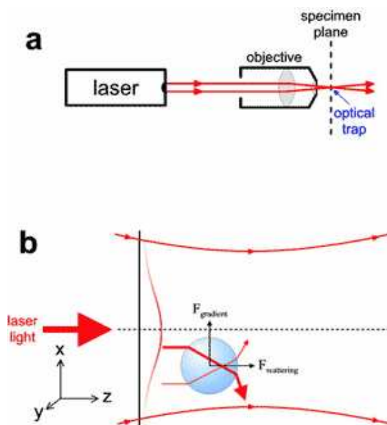
Figure 3: A single laser tweezers setup. (a) The laser light is focused into a spot by using an objective. (b) A Gaussian profile of light intensity generates a confining potential due to conservation of light momentum. The trapping force is induced by the difference in the index of refraction between the polystyrene bead and the surrounding water.
