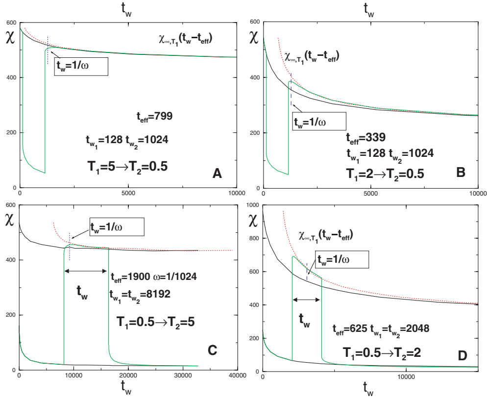
Figure 8. Negative and positive temperature cycles. (A) and (B) correspond to cycles with \Delta T < 0 , data for \omega = 1/128 , t_{w_1} = 128 , t_{w_2} = 1024 and for cycle (A): T_1 = 5 , T_2 = 0.5 and (B): T_1 = 2 , T_2 = 0.5 . (C) and (D) correspond to cycles with \Delta T > 0 , for cycle (C): T_1 = 0.5 , T_2 = 5 , \omega = 1/1024 and t_{w_1} = t_{w_2} = 8192 and (D): T_1 = 0.5 , T_2 = 2 , \omega = 1/1024 and t_{w_1} = t_{w_2} = 2048 . The dashed line corresponds to the first measurement possible in a regular experiment t_w = 1/\omega .
