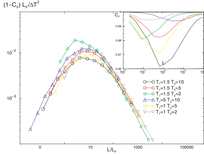
Figure 2. Scaling function for the free-energy correlations. (1 - C_F) \times \frac{\sigma^2 L_F^*}{\Delta T^2} as a function of \frac{L}{L_F} for different pairs of temperatures (T_1, T_2) .
